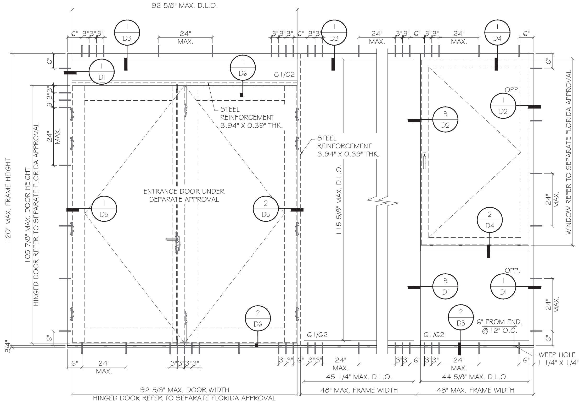
YY150T TYPICAL EXTERIOR ELEVATION MAX. DESIGN LOAD: +/- 60 PSF
