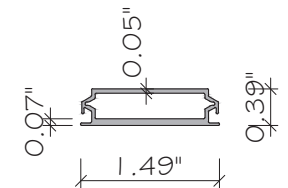
E21 COVER PLATE ALUMINUM. 6063-T5
