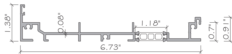
E25 SUBSILL ALUMINUM. 6063-T5
