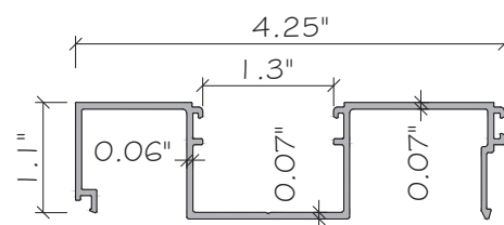
E8 GLASS BEAD FOR CURVE FRAME ALUMINUM. 6063-T5
