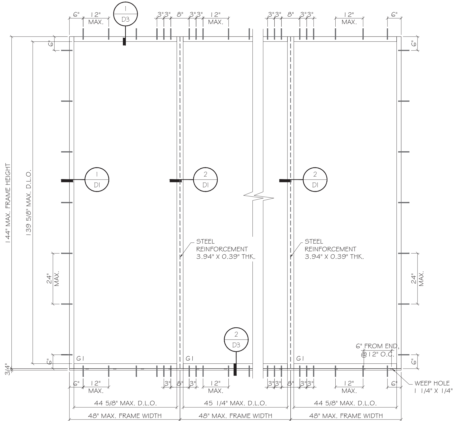
YY150T TYPICAL EXTERIOR ELEVATION MAX. DESIGN LOAD: +/- 60 PSF
